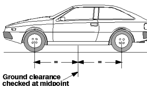
Ground clearance at the mid-point between 2 axles
