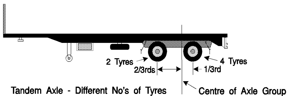
Tandem Axle - Different No's of Tyres Centre line of a tandem axle group fitted with a different number of tyres on each axle
