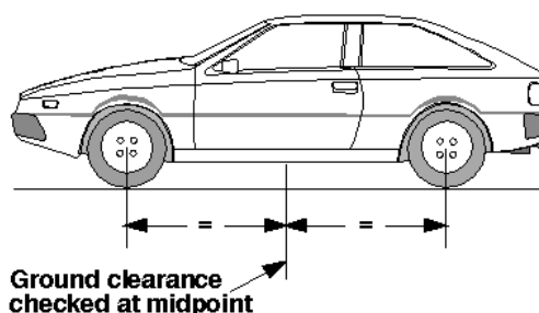
Ground clearance at the mid-point between 2 axes
